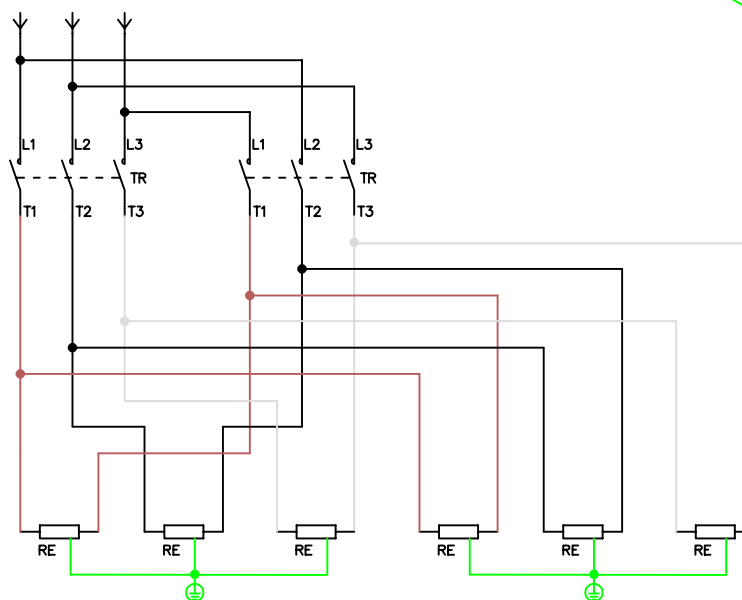
6 RESISTENZE/HEATING ELEMENTS 3ph 208V-240V 50/60Hz
