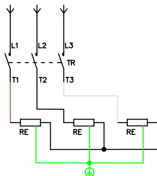
3 RESISTENZE/HEATING ELEMENTS 3ph (+N) 380V-440V 50/60Hz
