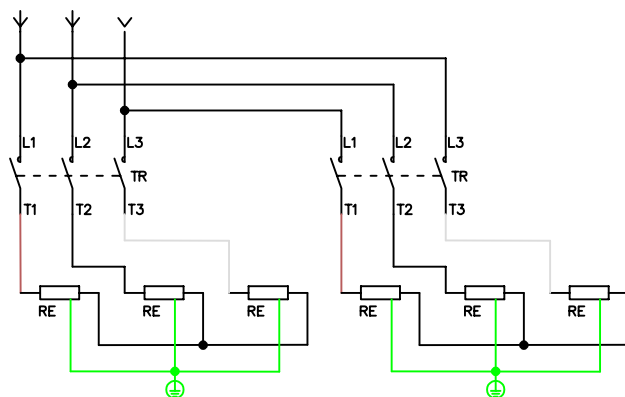
6 RESISTENZE/HEATING ELEMENTS 3ph (+N) 380V-440V 50/60Hz
