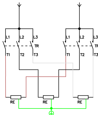
3 RESISTENZE/HEATING ELEMENTS 1ph 208V-240V 50/60Hz
